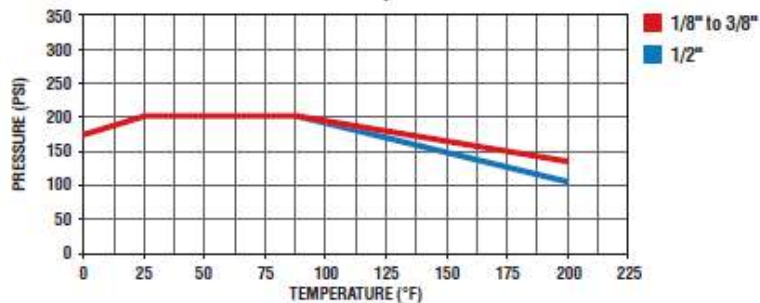
MV200 Pressure and Temperature
