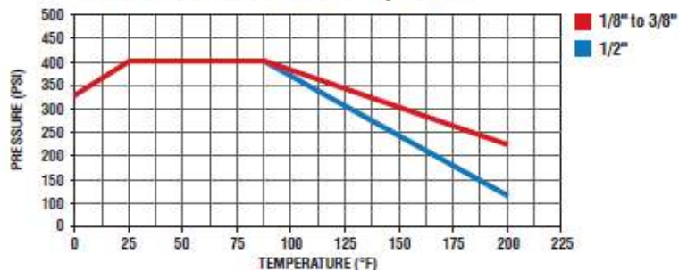
MV608/609 Pressure and Temperature
